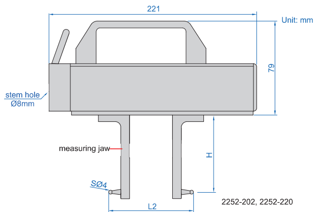
measure internal diameter 2252-220
