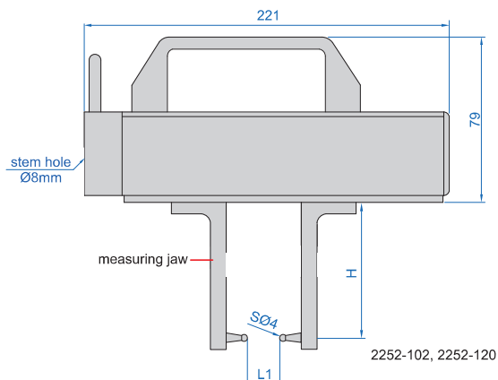
measure external diameter 2252-120
